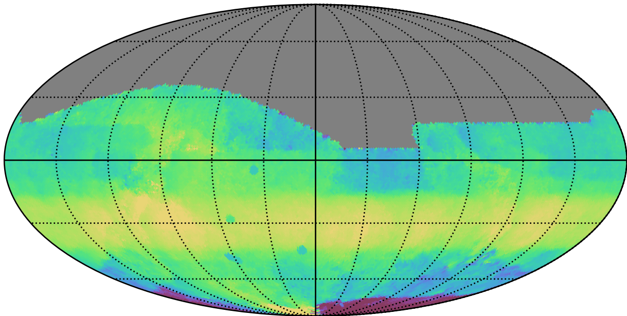
ddf_half_v3.4_10yrs All sky i band: Median HA
