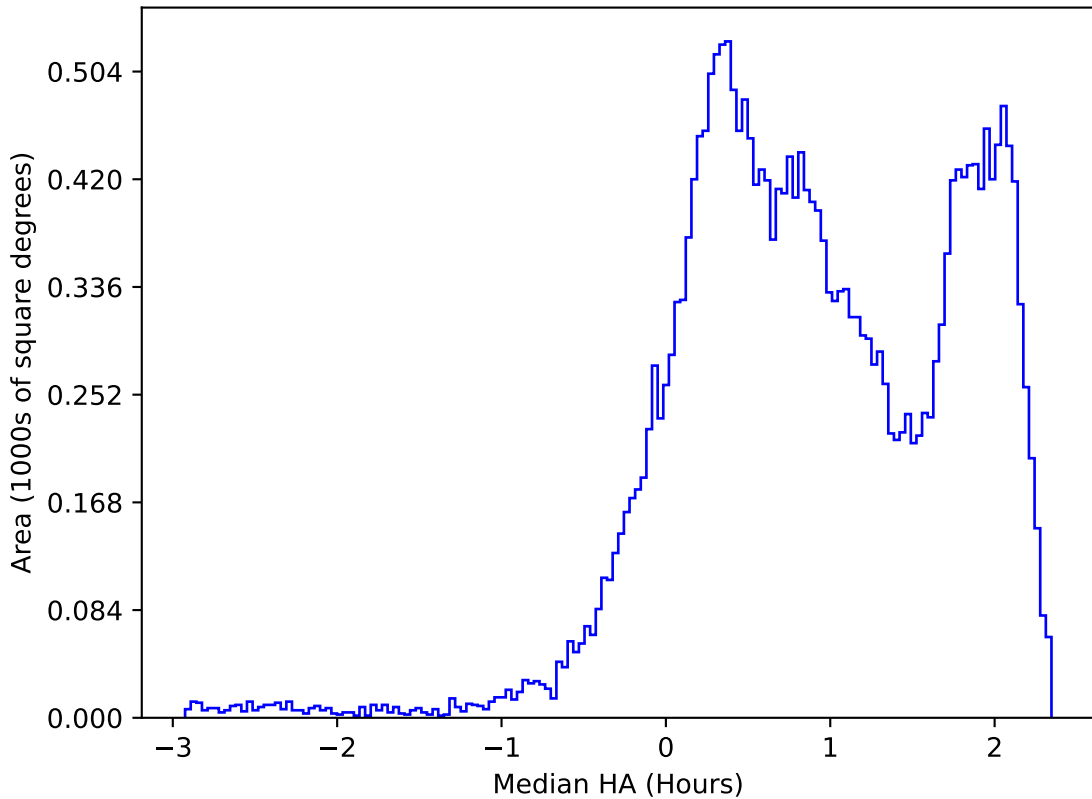
ddf_half_v3.4_10yrs All sky i band: Median HA
