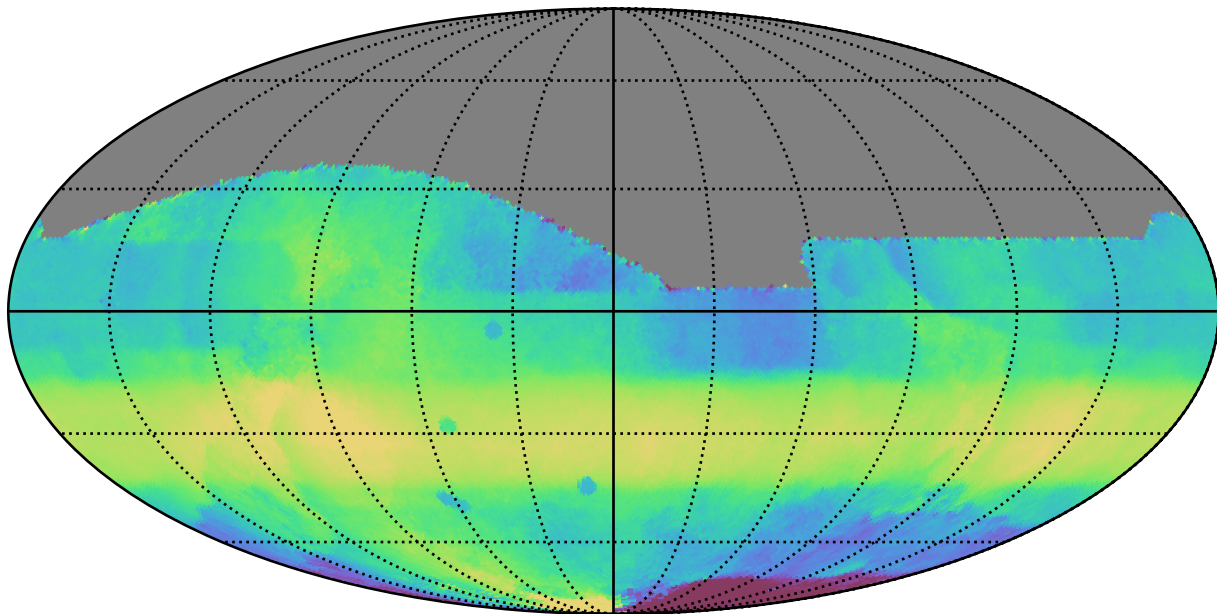
ddf_half_v3.4_10yrs All sky all bands: Median HA
