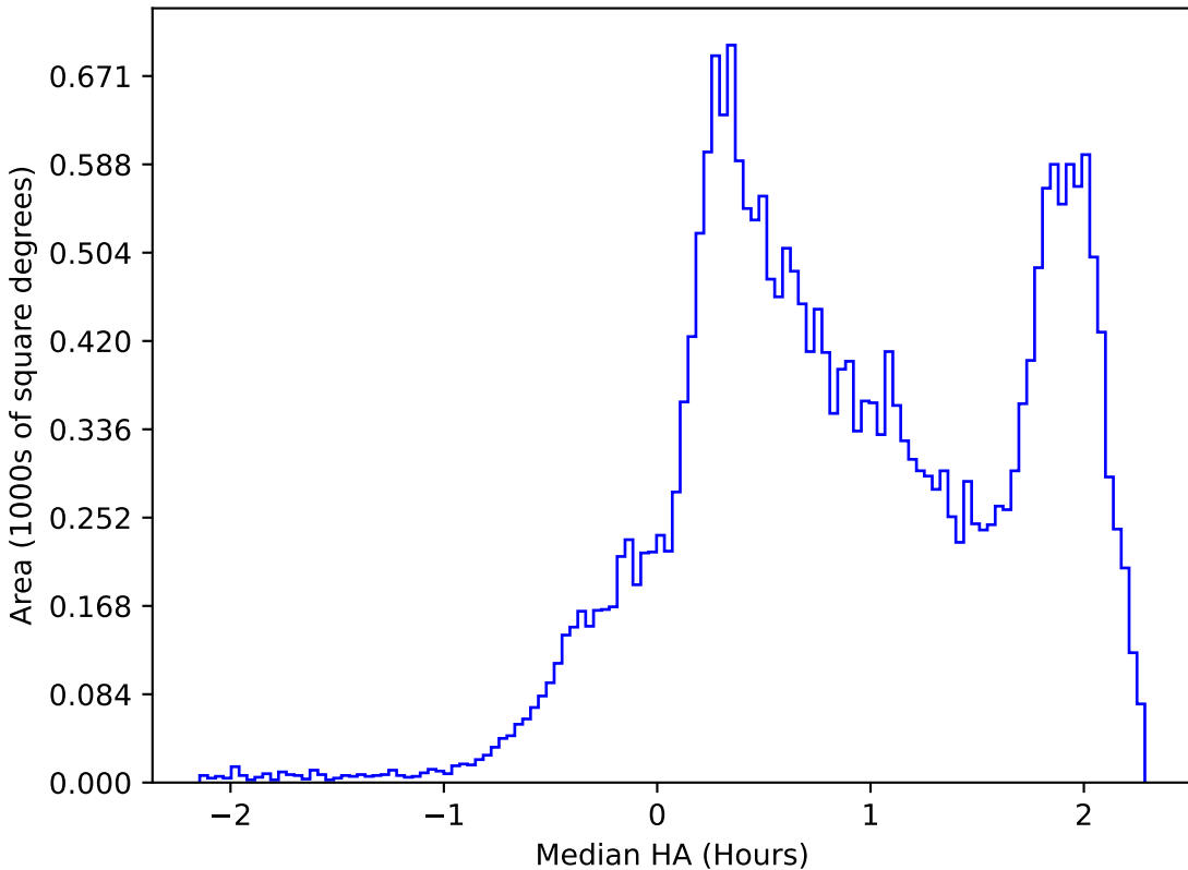
ddf_half_v3.4_10yrs All sky all bands: Median HA
