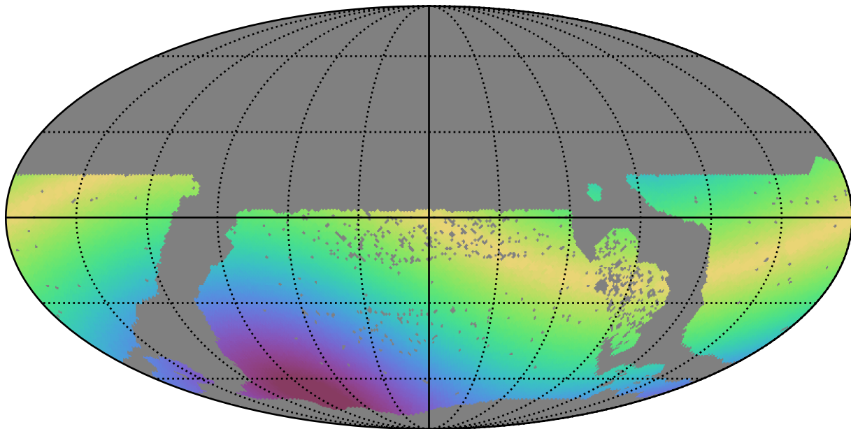
ddf_half_v3.4_10yrs WFD z band: Max solarElong
