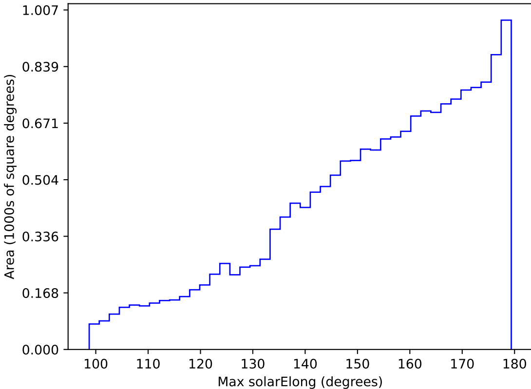
ddf_half_v3.4_10yrs WFD z band: Max solarElong
