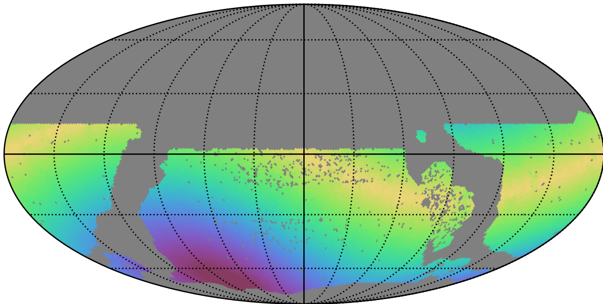
ddf_half_v3.4_10yrs WFD u band: Max solarElong
