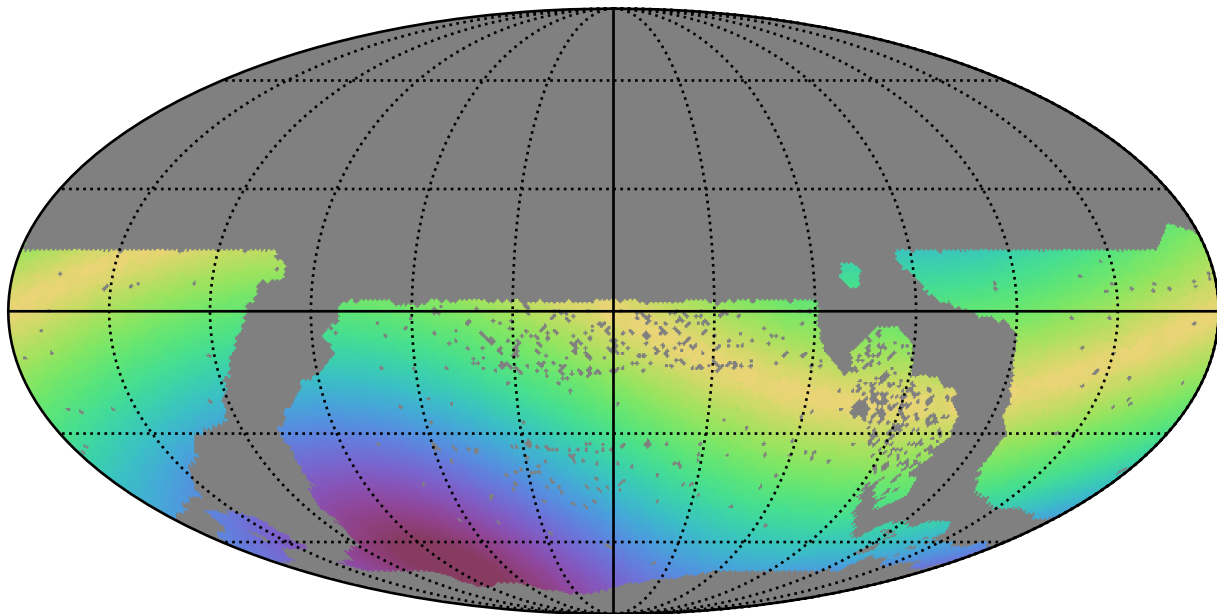
ddf_half_v3.4_10yrs WFD r band: Max solarElong
