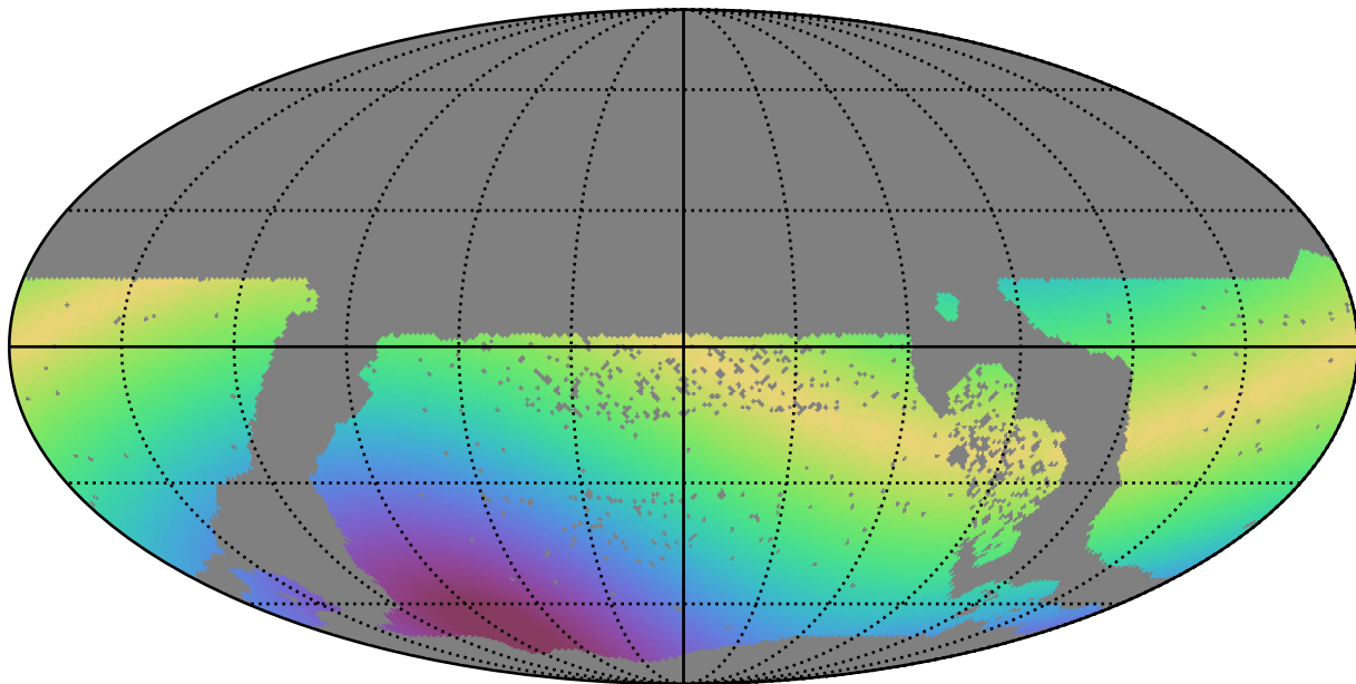
ddf_half_v3.4_10yrs WFD i band: Max solarElong
