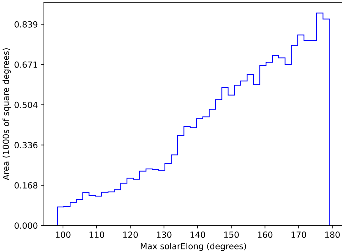
ddf_half_v3.4_10yrs WFD g band: Max solarElong
