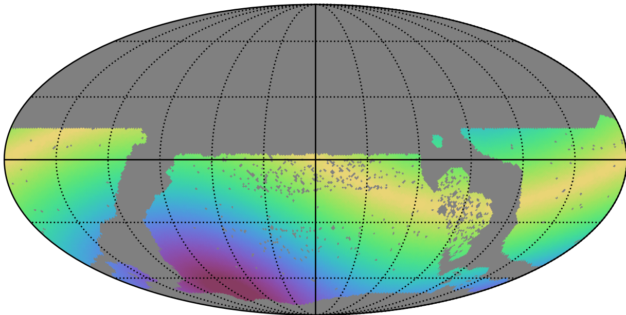
ddf_half_v3.4_10yrs WFD all bands: Max solarElong
