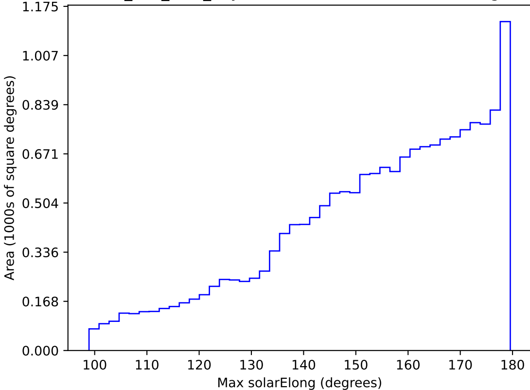
ddf_half_v3.4_10yrs WFD all bands: Max solarElong
