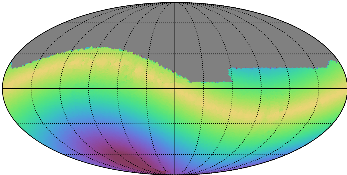
ddf_half_v3.4_10yrs All sky z band: Max solarElong
