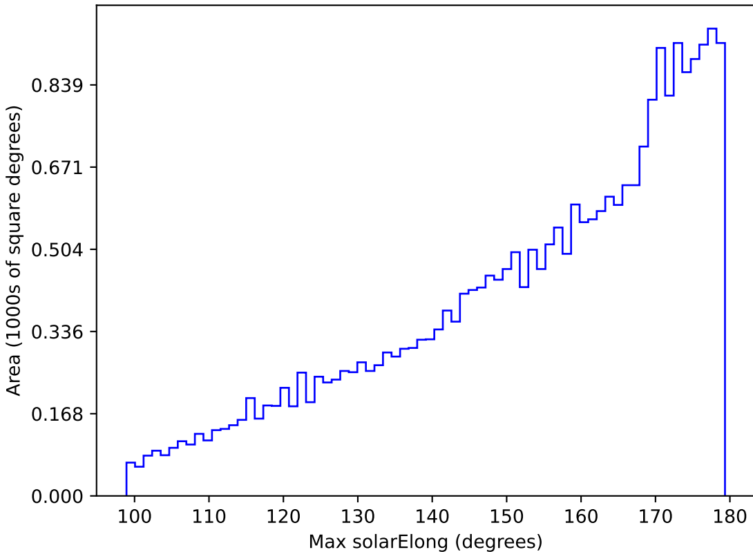
ddf_half_v3.4_10yrs All sky z band: Max solarElong
