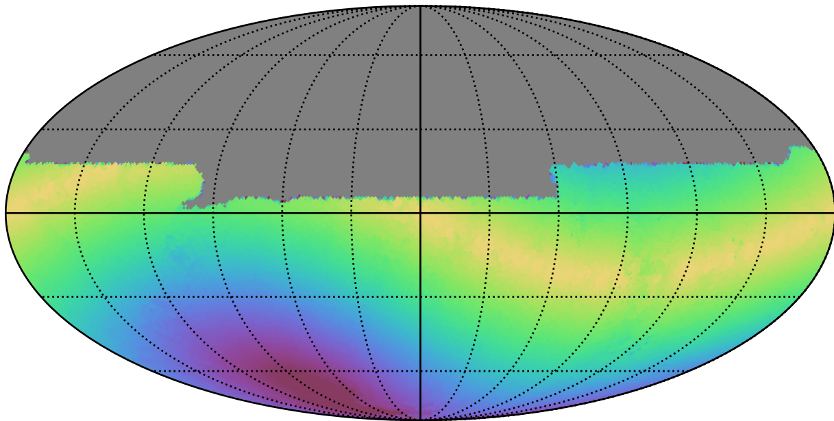
ddf_half_v3.4_10yrs All sky u band: Max solarElong
