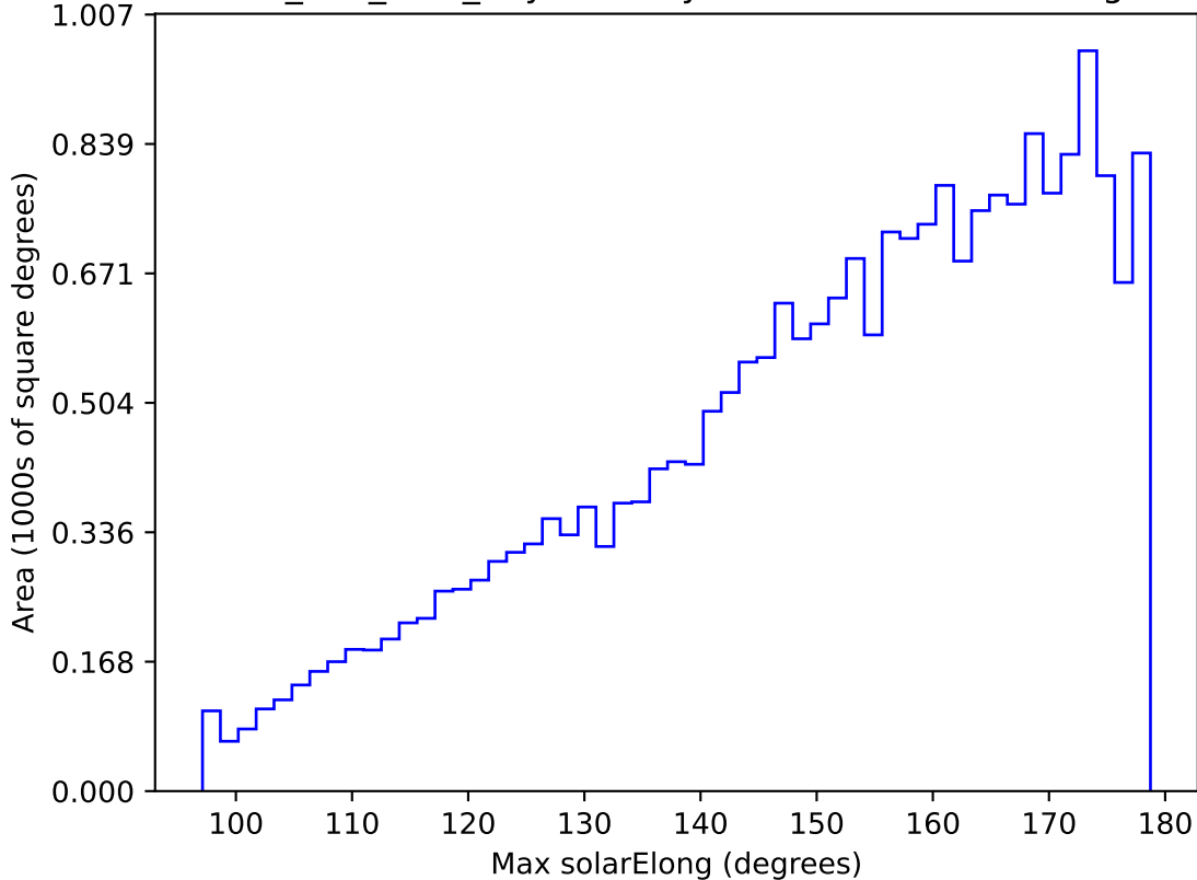
ddf_half_v3.4_10yrs All sky u band: Max solarElong
