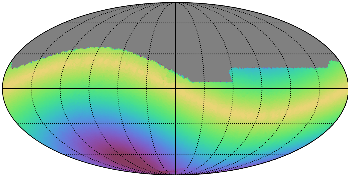
ddf_half_v3.4_10yrs All sky r band: Max solarElong
