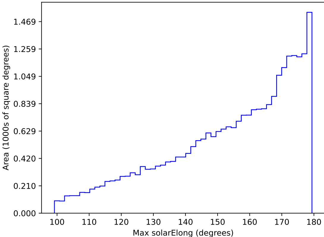
ddf_half_v3.4_10yrs All sky r band: Max solarElong
