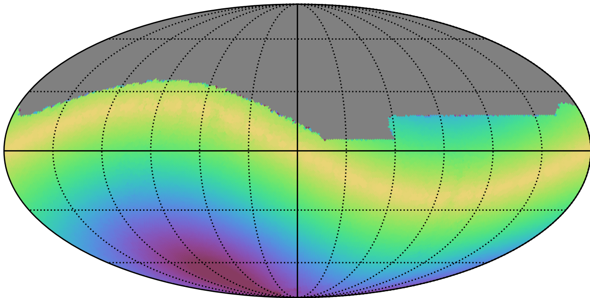
ddf_half_v3.4_10yrs All sky i band: Max solarElong
