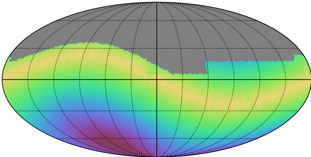
ddf_half_v3.4_10yrs All sky g band: Max solarElong
