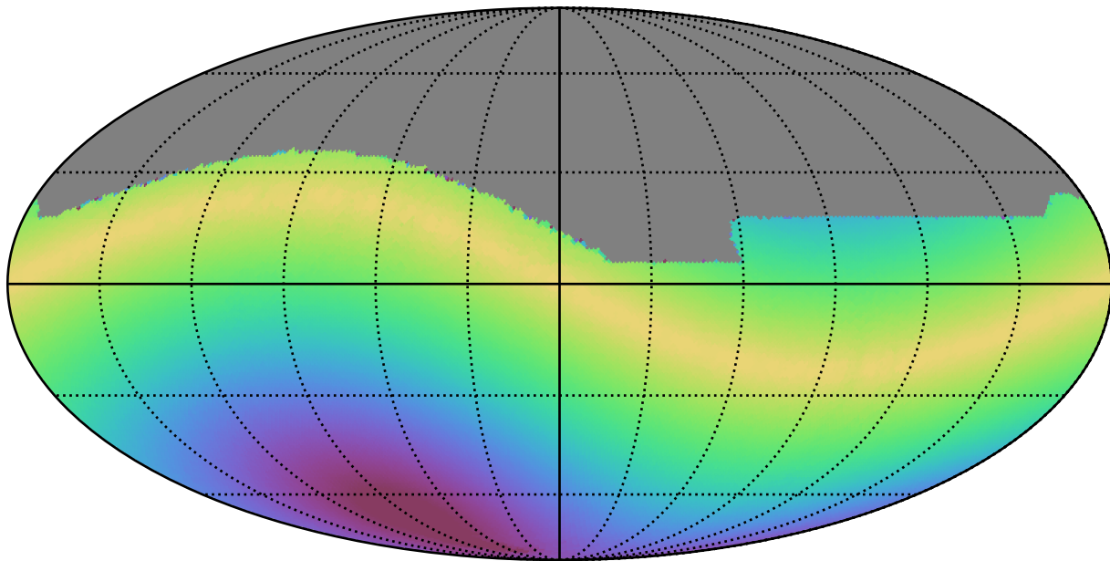
ddf_half_v3.4_10yrs All sky all bands: Max solarElong
