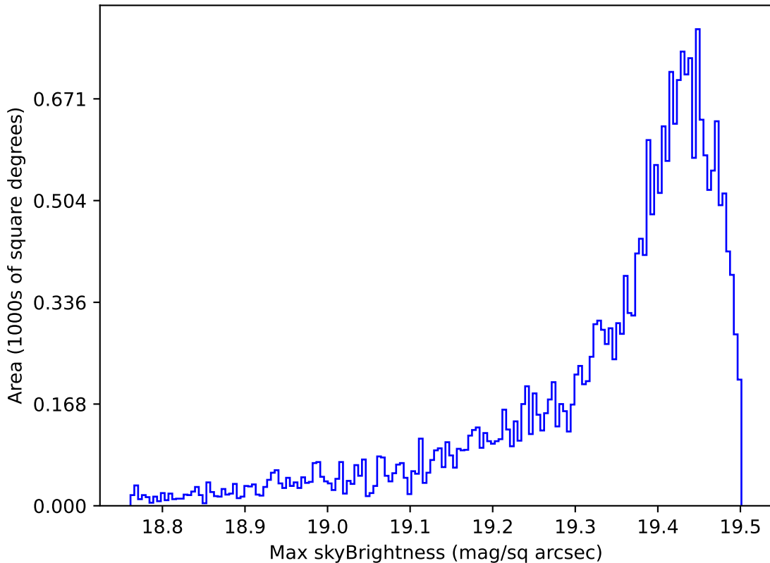
ddf_half_v3.4_10yrs Yr 1 z band: Max skyBrightness
