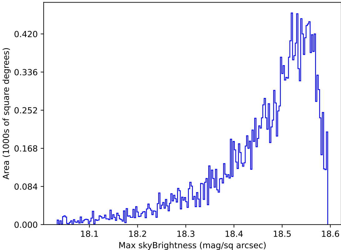
ddf_half_v3.4_10yrs Yr 1 y band: Max skyBrightness
