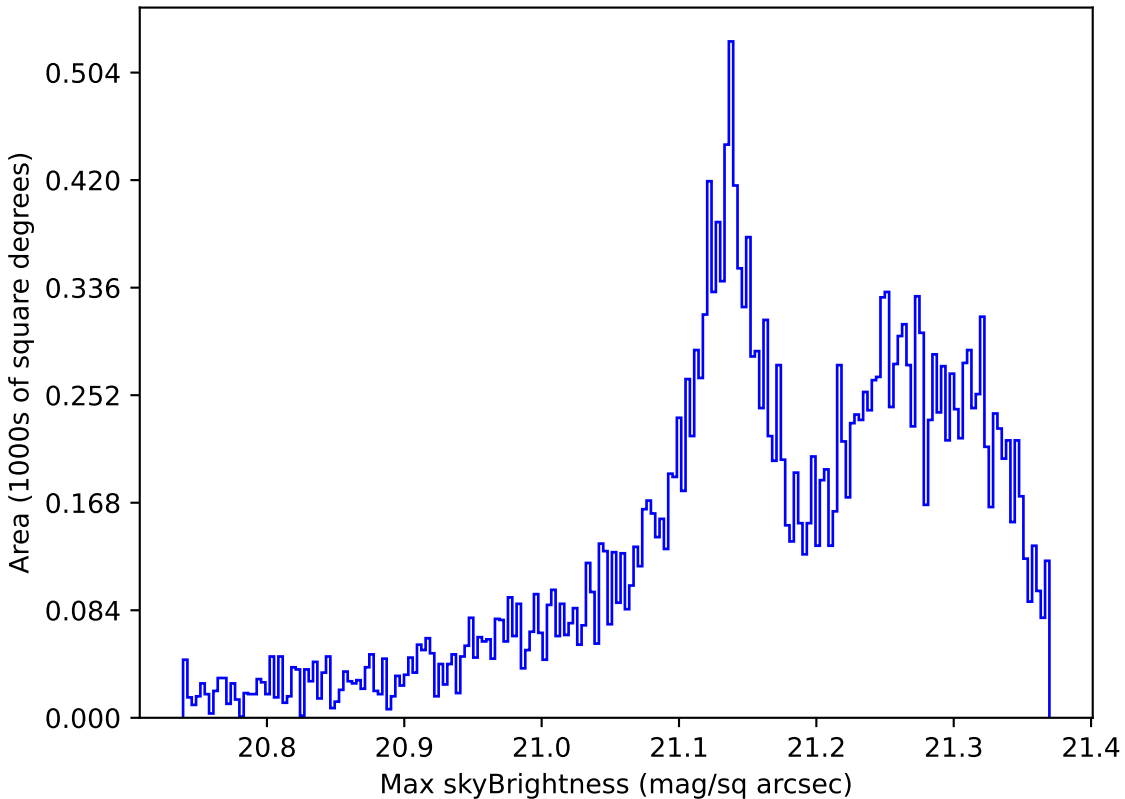
ddf_half_v3.4_10yrs Yr 1 r band: Max skyBrightness
