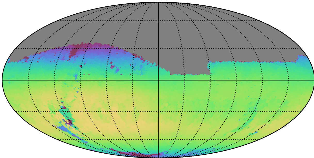
ddf_half_v3.4_10yrs Yr 1 i band: Max skyBrightness
