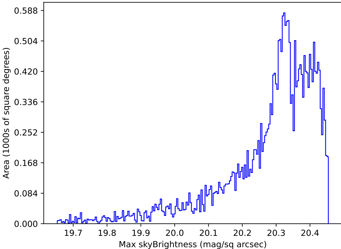
ddf_half_v3.4_10yrs Yr 1 i band: Max skyBrightness
