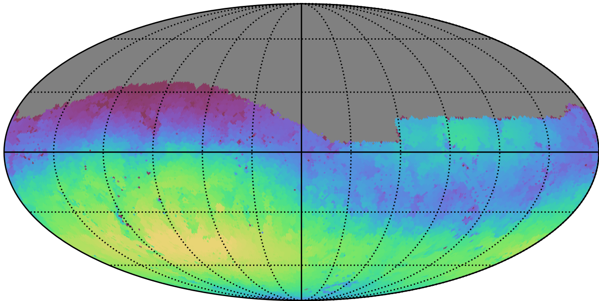
ddf_half_v3.4_10yrs Yr 1 g band: Max skyBrightness
