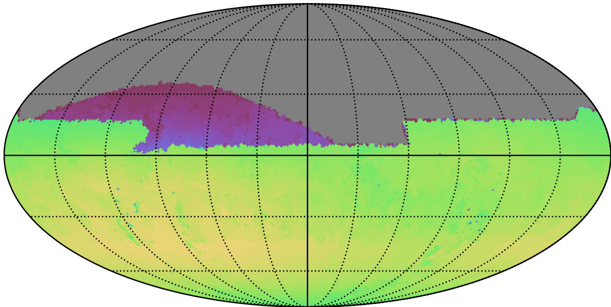
ddf_half_v3.4_10yrs Yr 1 all bands: Max skyBrightness
