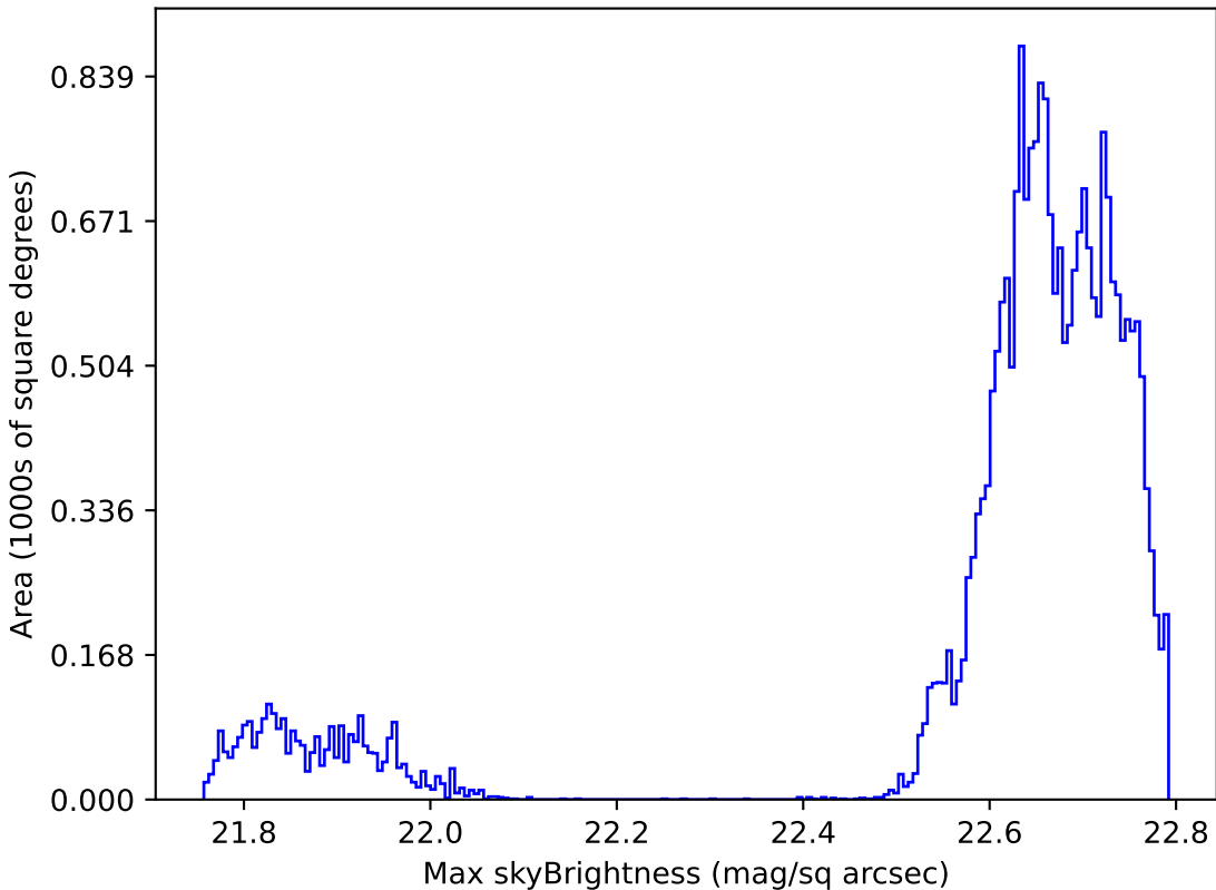
ddf_half_v3.4_10yrs Yr 1 all bands: Max skyBrightness
