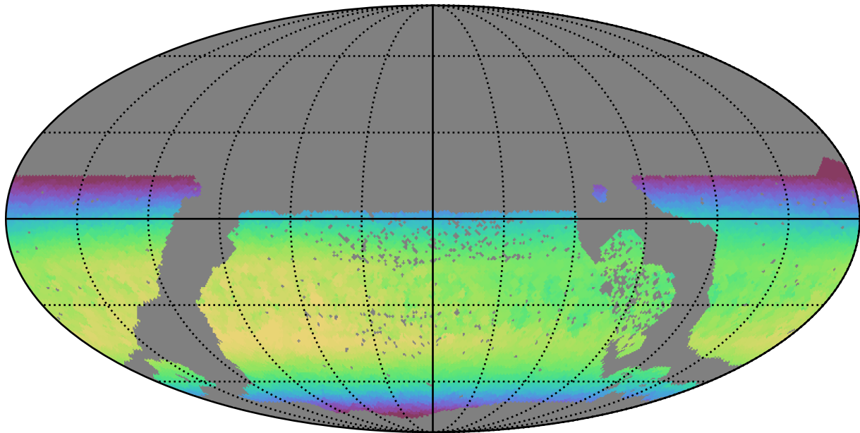
ddf_half_v3.4_10yrs WFD z band: Max skyBrightness
