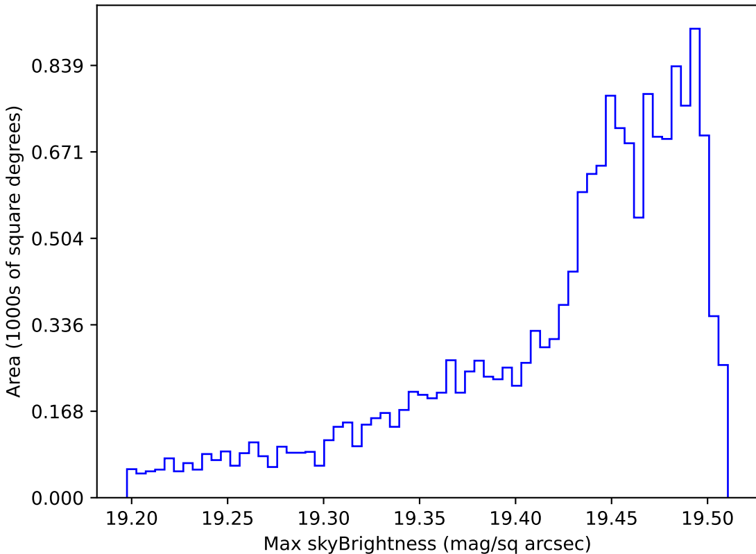
ddf_half_v3.4_10yrs WFD z band: Max skyBrightness
