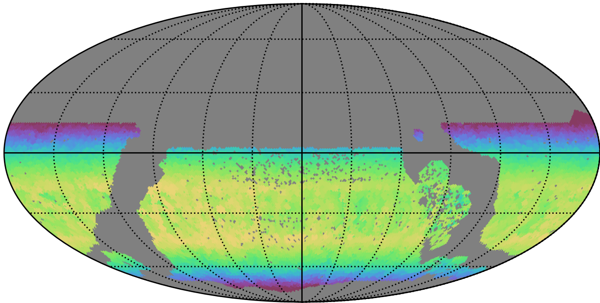
ddf_half_v3.4_10yrs WFD y band: Max skyBrightness
