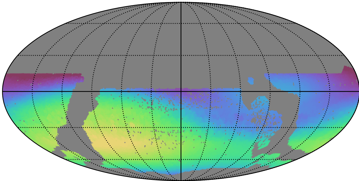
ddf_half_v3.4_10yrs WFD r band: Max skyBrightness
