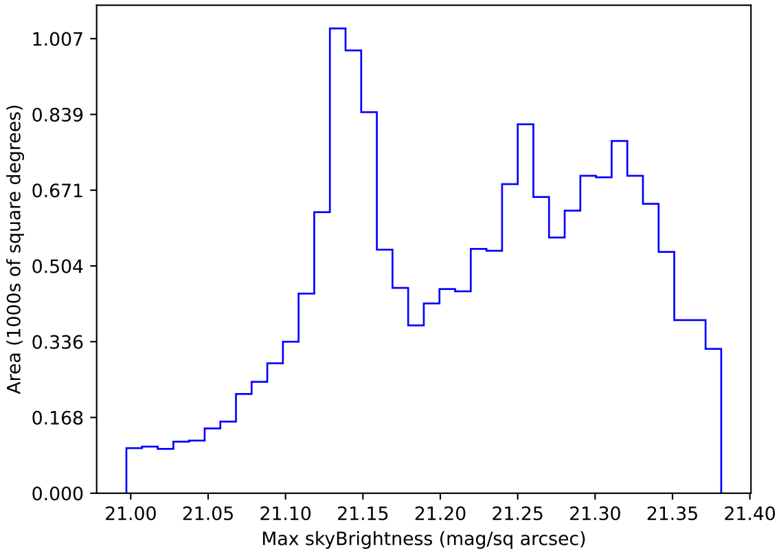
ddf_half_v3.4_10yrs WFD r band: Max skyBrightness
