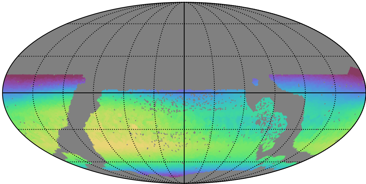
ddf_half_v3.4_10yrs WFD i band: Max skyBrightness
