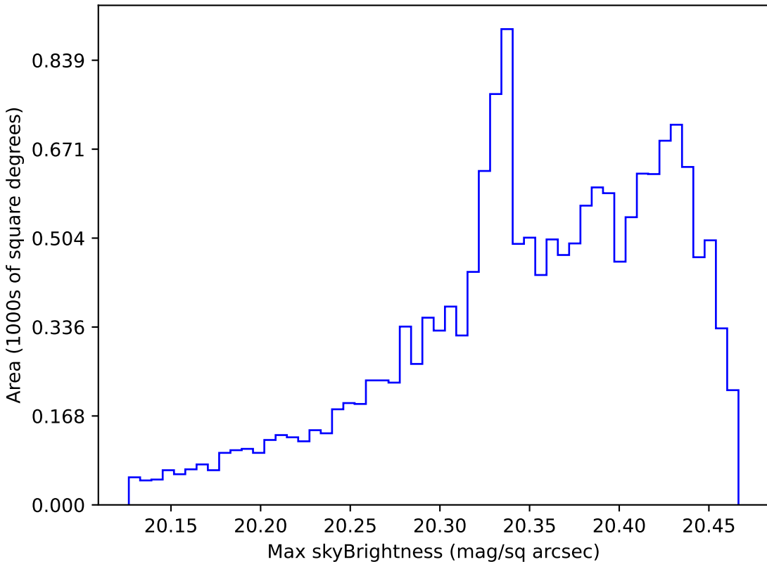
ddf_half_v3.4_10yrs WFD i band: Max skyBrightness
