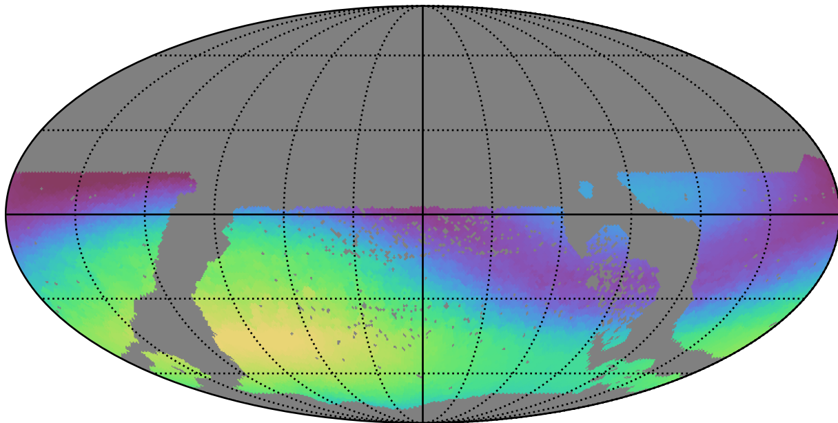
ddf_half_v3.4_10yrs WFD g band: Max skyBrightness
