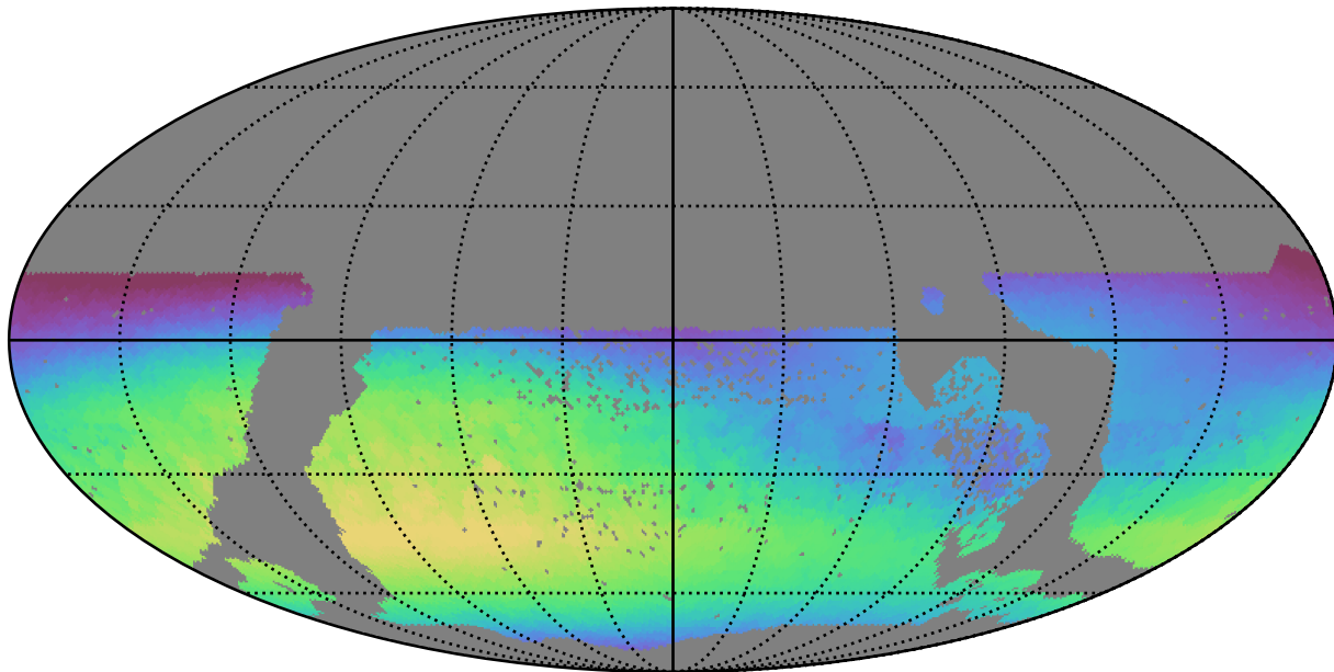
ddf_half_v3.4_10yrs WFD all bands: Max skyBrightness
