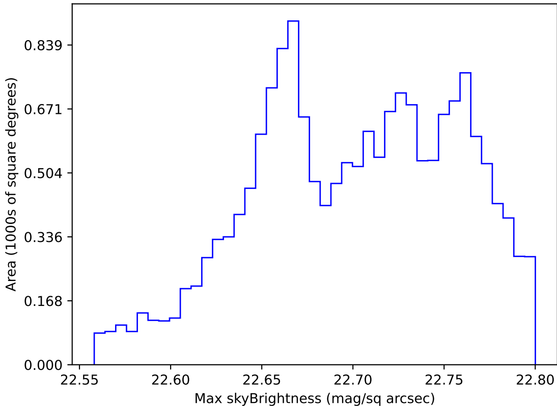
ddf_half_v3.4_10yrs WFD all bands: Max skyBrightness
