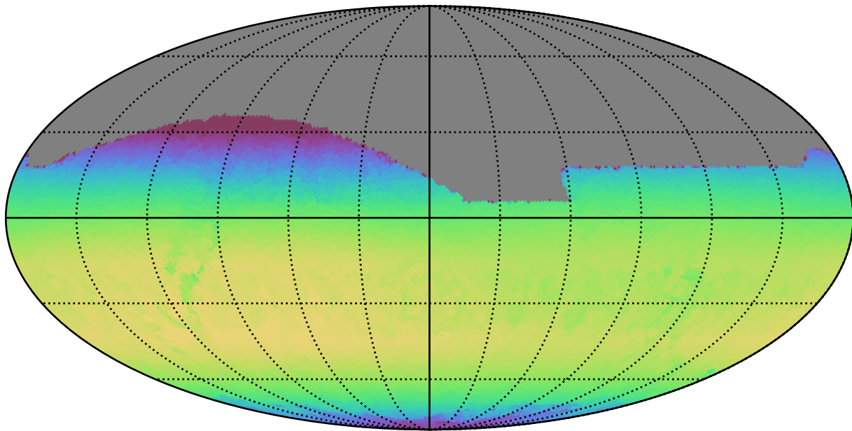
ddf_half_v3.4_10yrs All sky z band: Max skyBrightness
