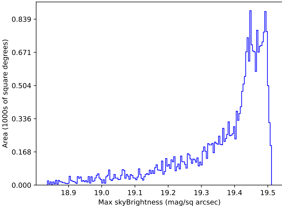
ddf_half_v3.4_10yrs All sky z band: Max skyBrightness
