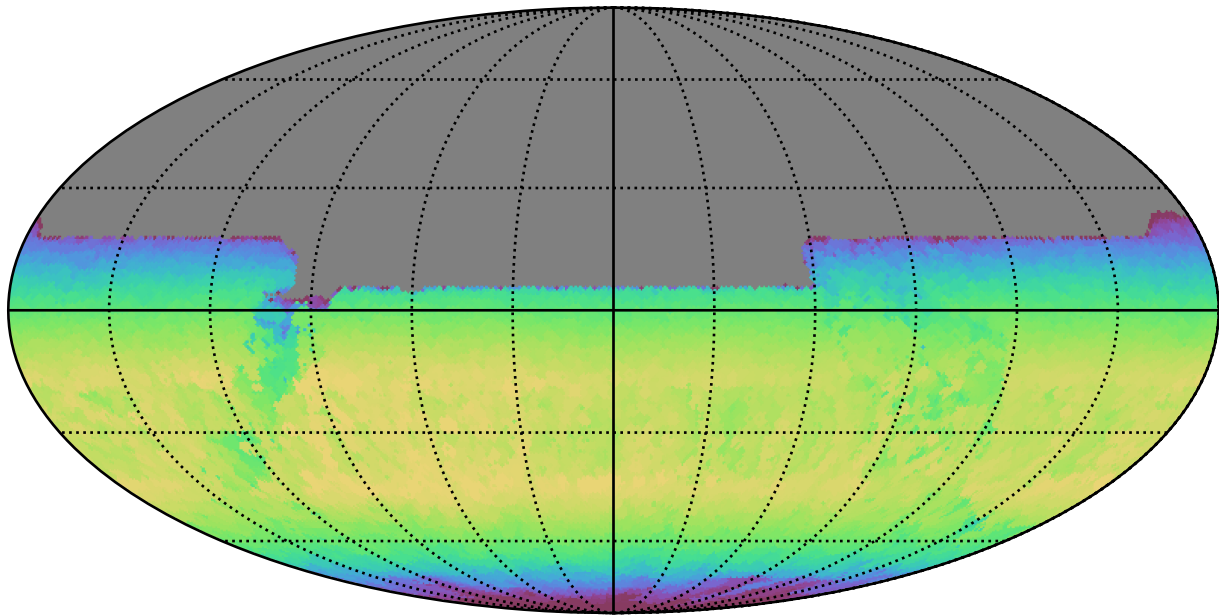
ddf_half_v3.4_10yrs All sky y band: Max skyBrightness
