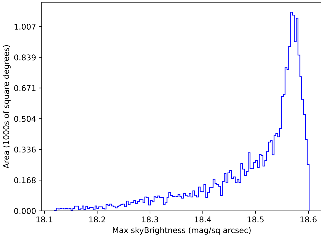
ddf_half_v3.4_10yrs All sky y band: Max skyBrightness
