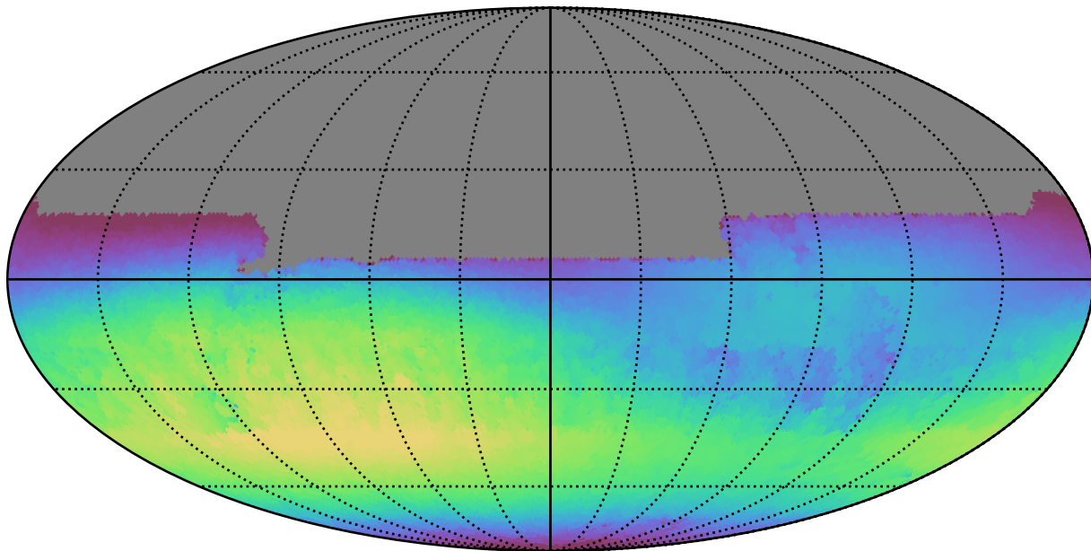
ddf_half_v3.4_10yrs All sky u band: Max skyBrightness
