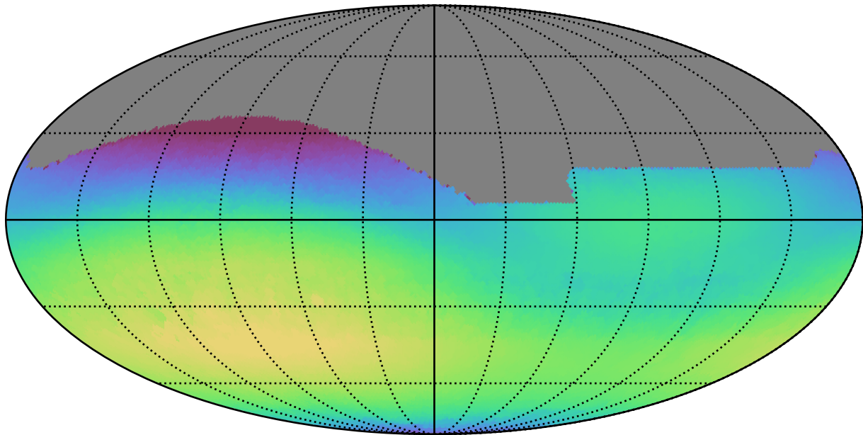
ddf_half_v3.4_10yrs All sky r band: Max skyBrightness
