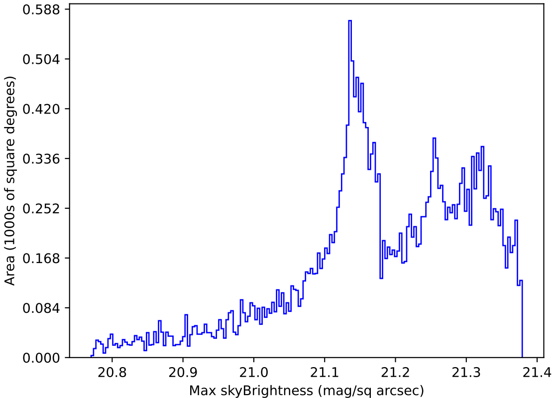
ddf_half_v3.4_10yrs All sky r band: Max skyBrightness
