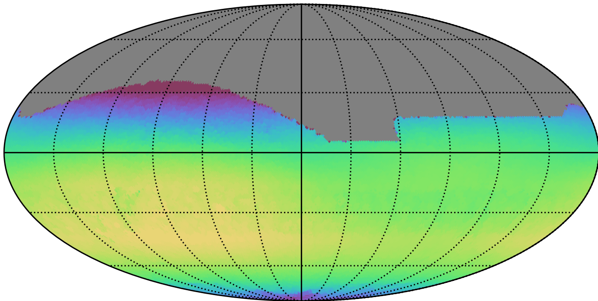
ddf_half_v3.4_10yrs All sky i band: Max skyBrightness
