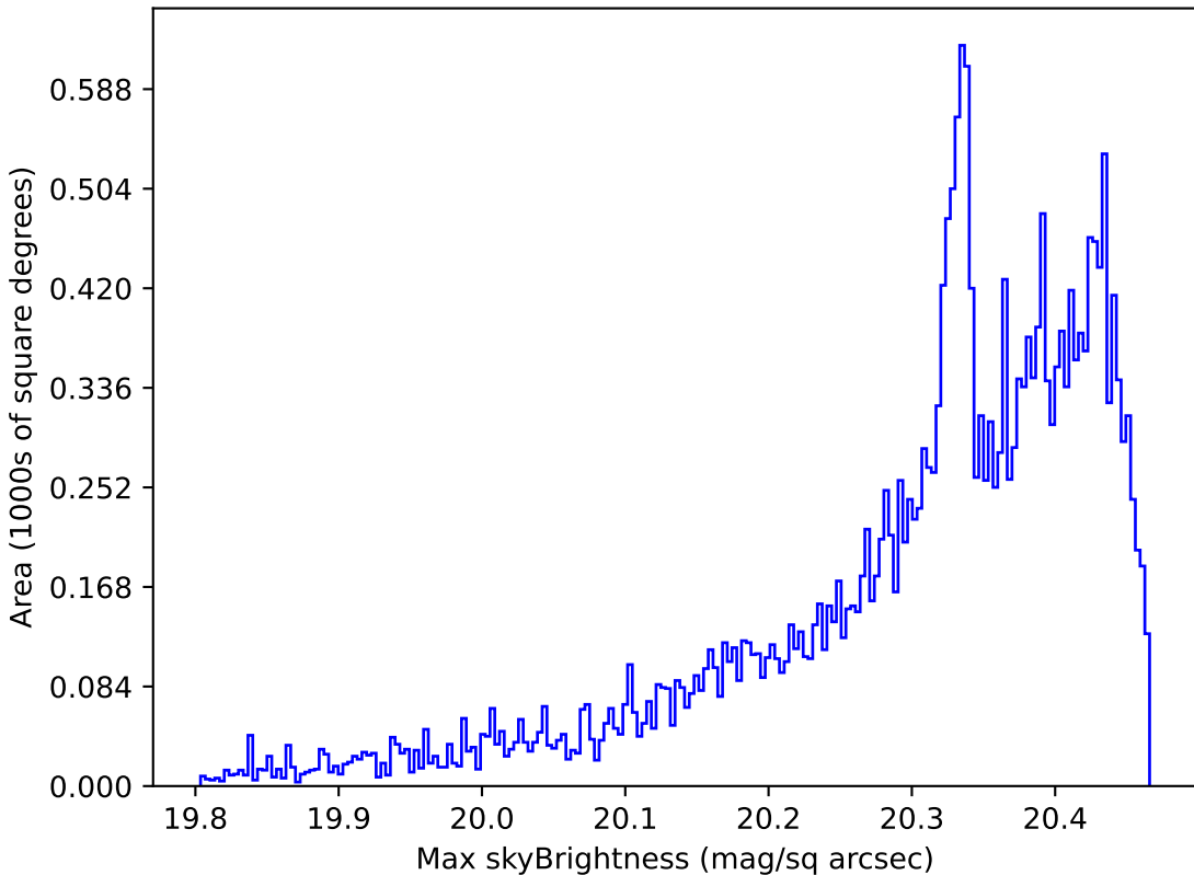
ddf_half_v3.4_10yrs All sky i band: Max skyBrightness
