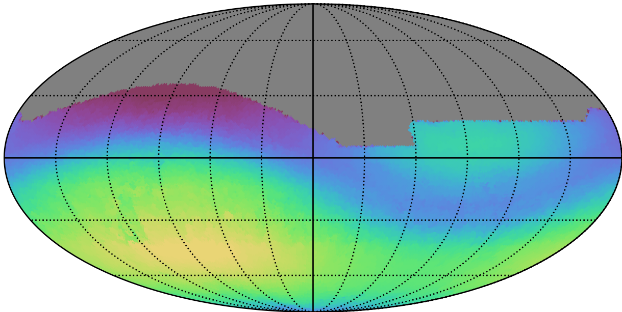
ddf_half_v3.4_10yrs All sky g band: Max skyBrightness
