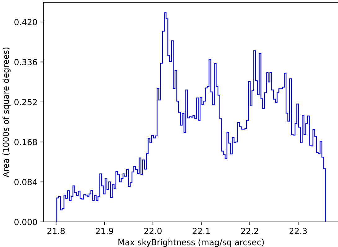
ddf_half_v3.4_10yrs All sky g band: Max skyBrightness
